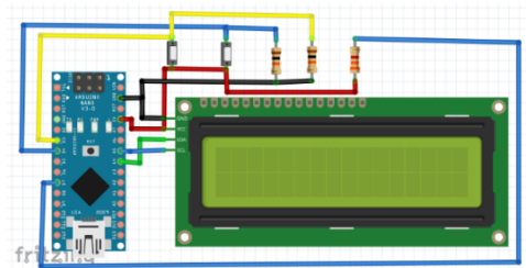
Figure 4: Breadboard diagram of circuit connection of digitalized part of thermal conductivity machine
