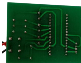
(e) Designed PCB Board back side
